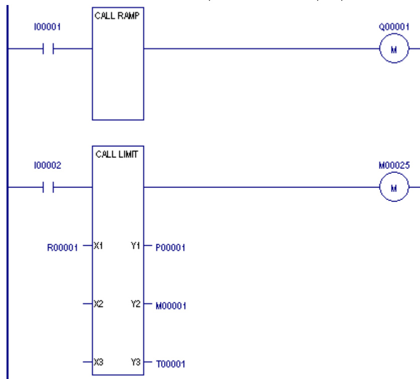
Figure 6: Ladder Logic Calls to C Blocks
