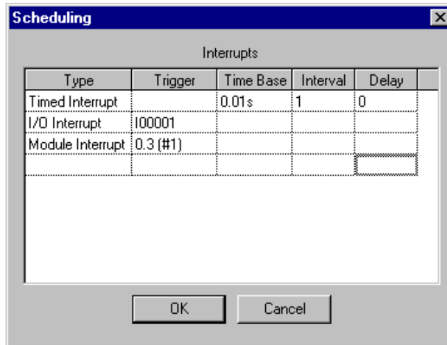
Figure 4: Scheduling a C Block
