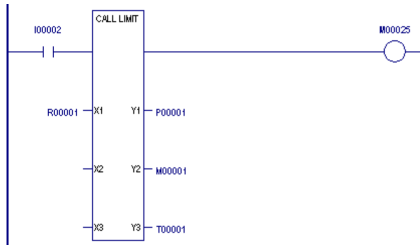
Figure 8: Reserving Space for Unused Parameters to a C Block
