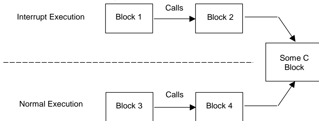
Figure 10: Interrupt Block Calls and C Blocks/FBKs
