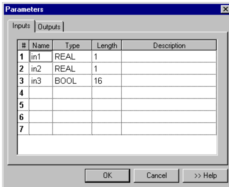
Figure 3: C Block Parameters in Properties Page
