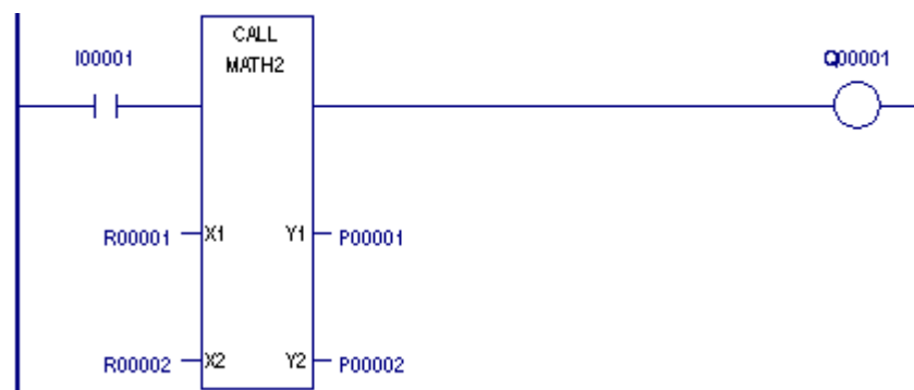
Figure 9: Importance of Matching Parameter Type, Order, and Number
