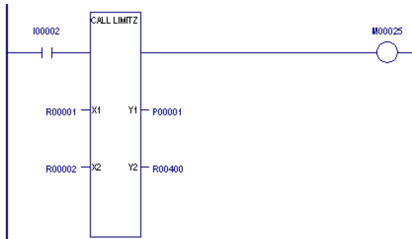
Figure 7: Matching Parameters Between Call and C Block
